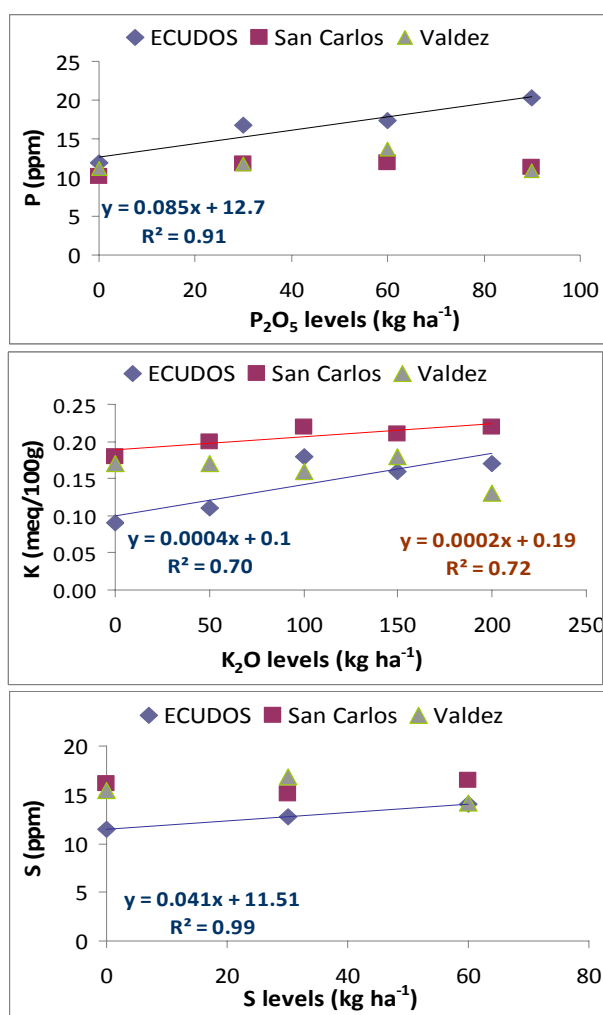
Fig. 1. Relationship between P 2 O 5 , K 2 O and S application and soil contents of P (ppm), K (meq/100 g soil) and S (ppm) evaluated in three locations, 2008.
