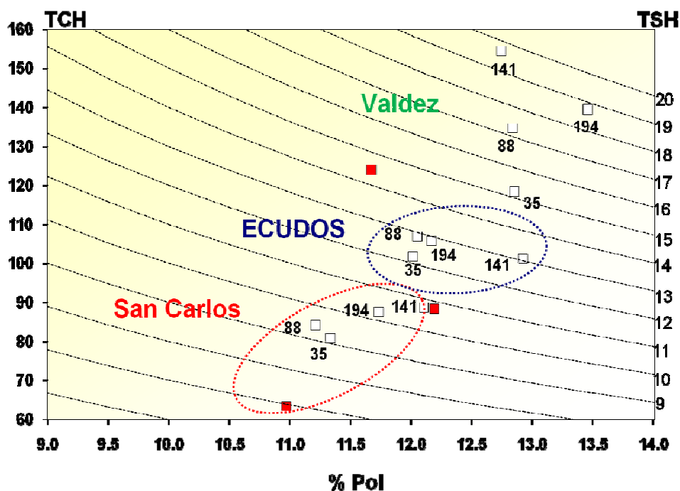
Fig. 2—Isoproductive lines of tonnage of cane/ha (TCH), tonnage of sugar/ha (TSH) and sugar concentration (% Pol) of variety ECU-01 in plant cane at four N levels (35, 88, 141 and 194 kg/ha) and 0 N control treatment (■). Data are from three locations in Ecuador.
